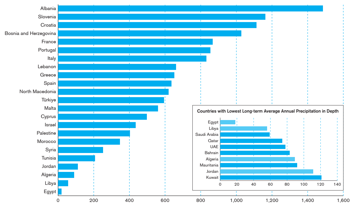
CHART F21 Long-term Average Annual Precipitation in Depth (mm/year)
