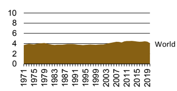
Evolution of GHG Emissions from Fuel Combustion by Country (1971-2020)
