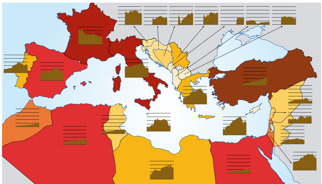
GHG Emissions from Fuel Combustion (million tonnes of CO 2 eq)
