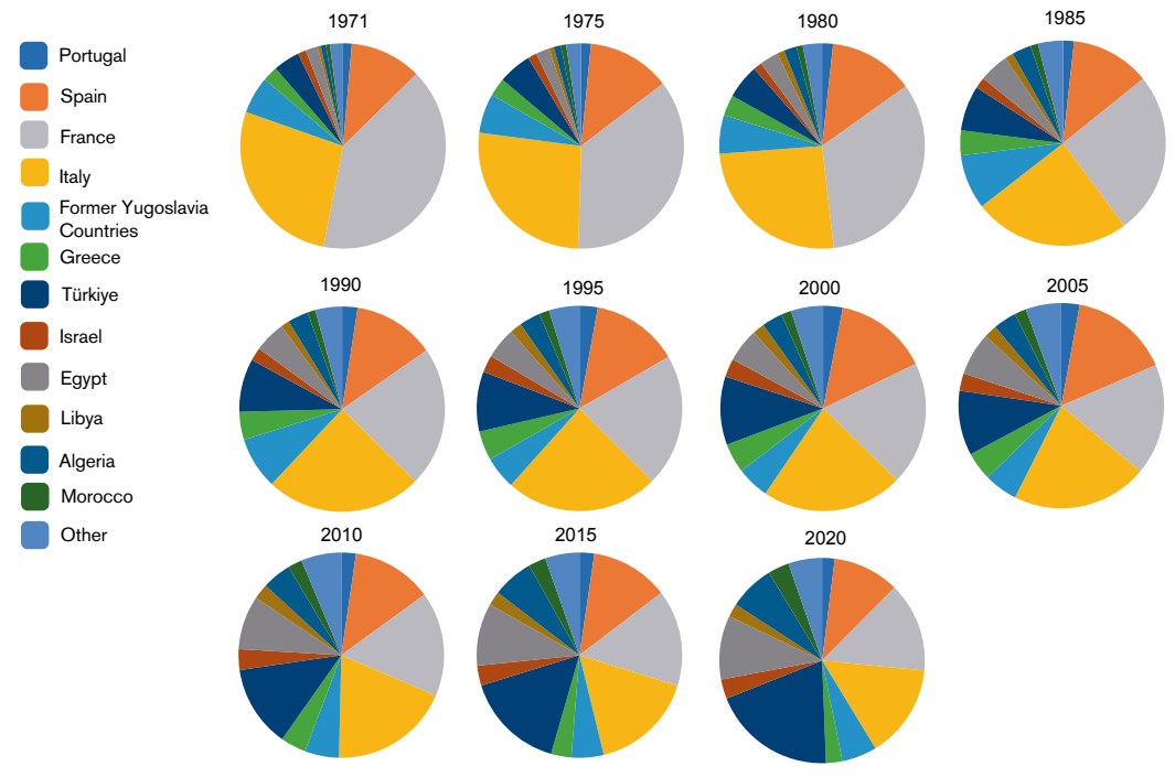
Evolution of GHG Emissions from Fuel Combustion by Country (1971-2020)
