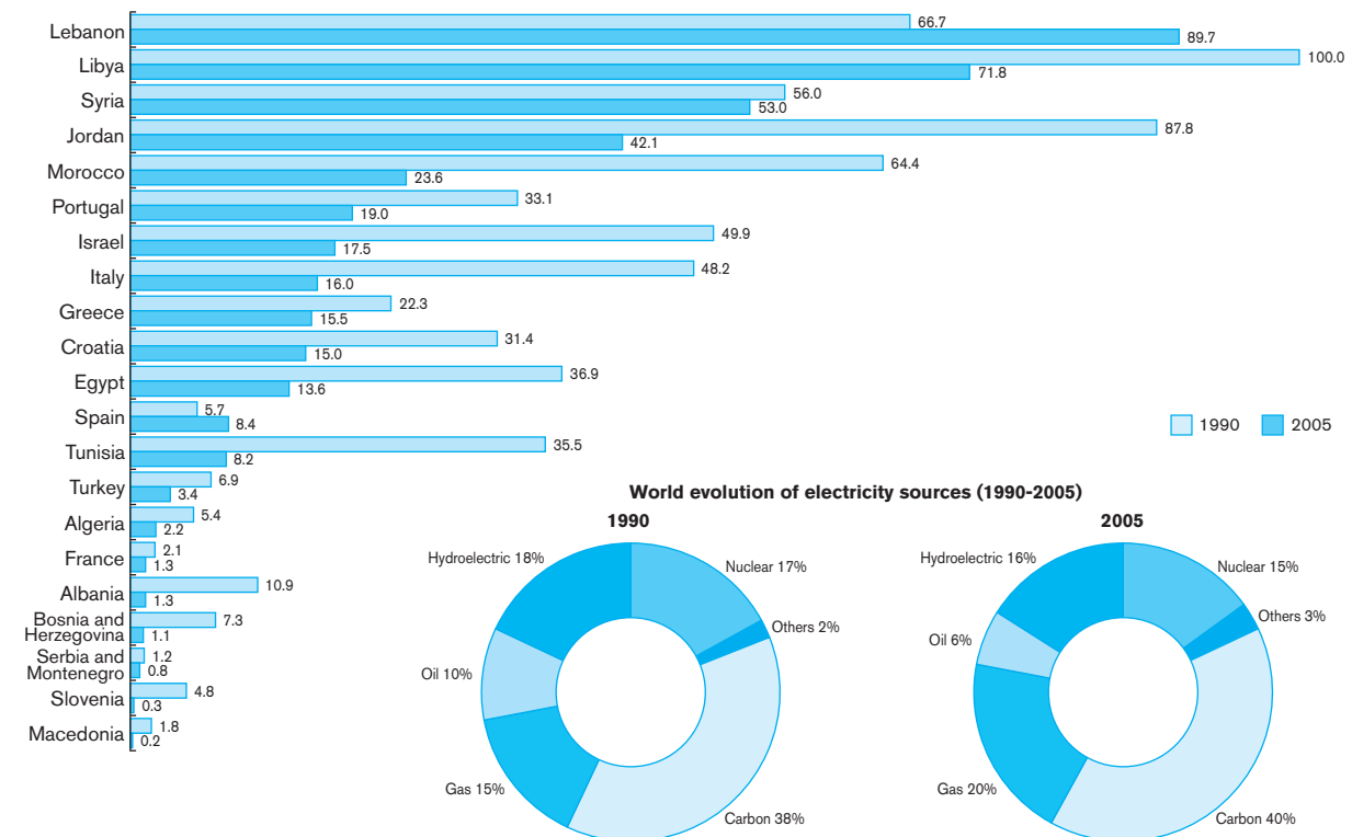
CHART F19 Share of oil in electricity generation* (1990-2005) (%)
