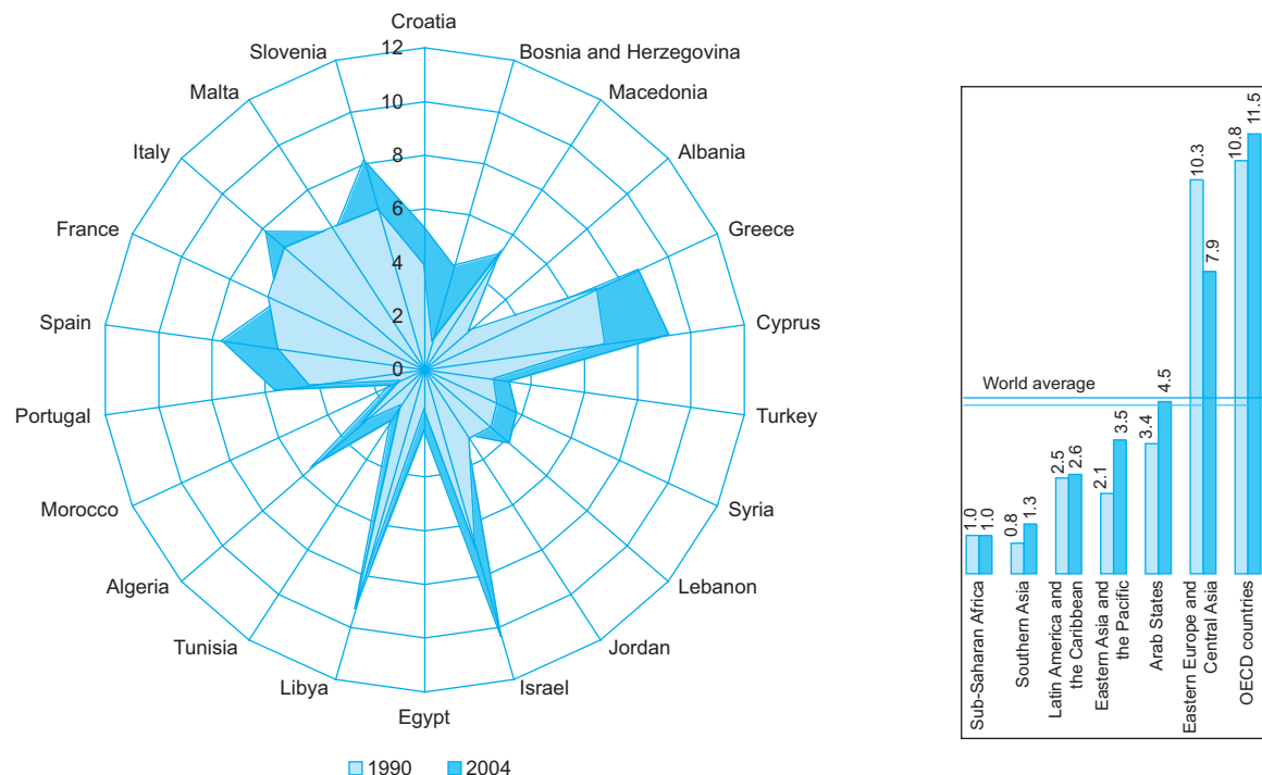
CHART F20 Evolution of per capita CO 2 emissions (mt) (1990-2004)
