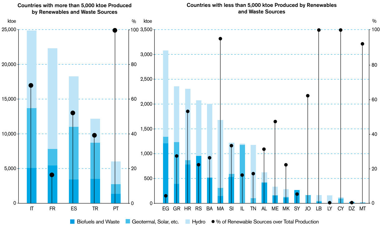
CHART F18 Energy Production by Renewables and Waste Sources (2014)
