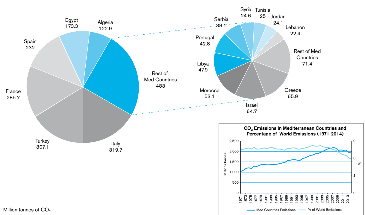
CHART F20 CO 2 Emissions in Mediterranean Countries. Share by Country (2014)
