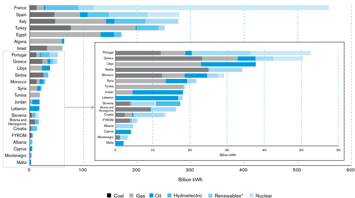
CHART F19 Electricity Consumption by Source (2014)
