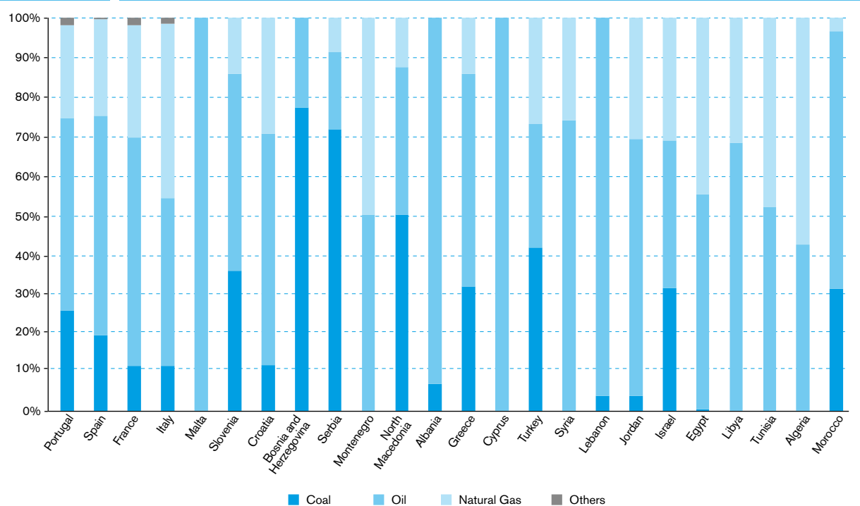
CHART F20 CO 2 Emissions by Energy Source (2017)
